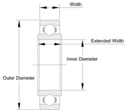
Bearing With Extended Inner Ring
